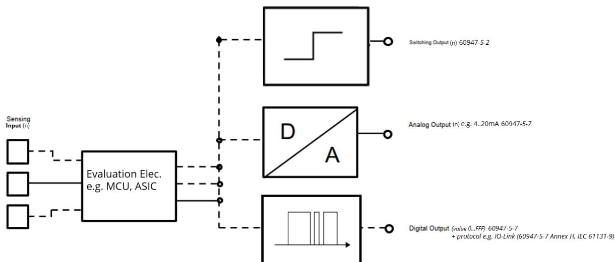
Figure 1 – Proximity device with analogue output, schematic block diagram structure
