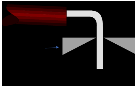
Figure 5-1: Profile of correct cutters for trimming leads
