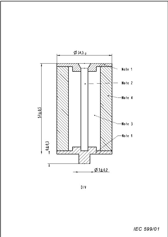
Dimensions in millimetres Figure 104 – Dummy fuse-links according to 8.3 and 8.9.1.1
