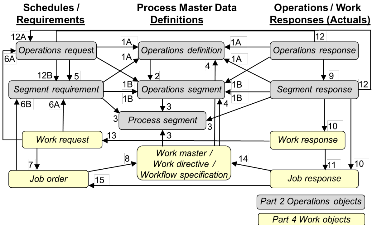
Figure 4 – Defined cross-model MOM relationships between operations & work models
