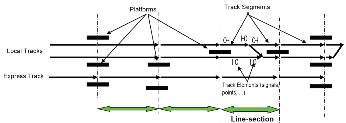
Figure 4 – UGTMS concept of line section
