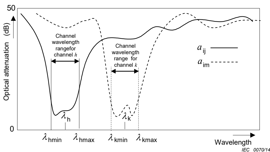
Figure 1 – Illustration of channel wavelength range
