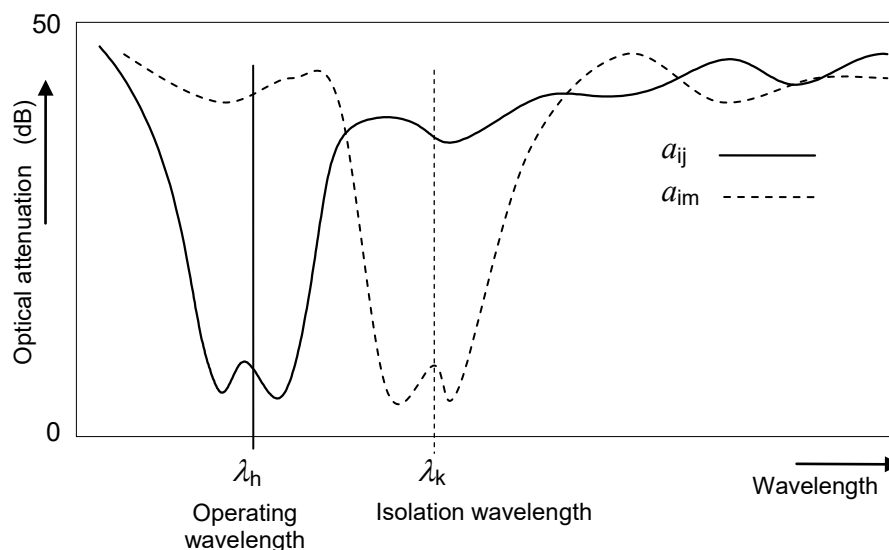
Figure 5 – Illustration of isolation wavelength
