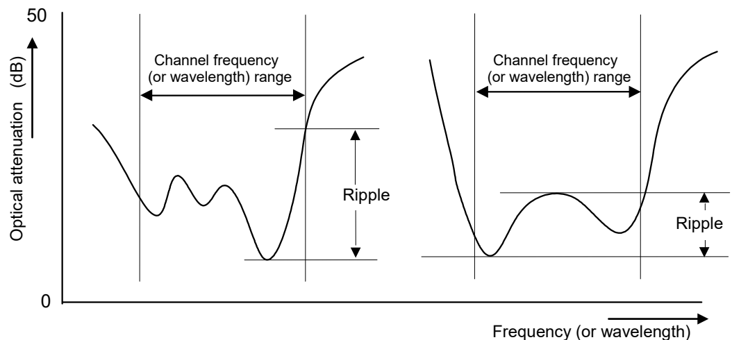
a) – Ripple at band edges
