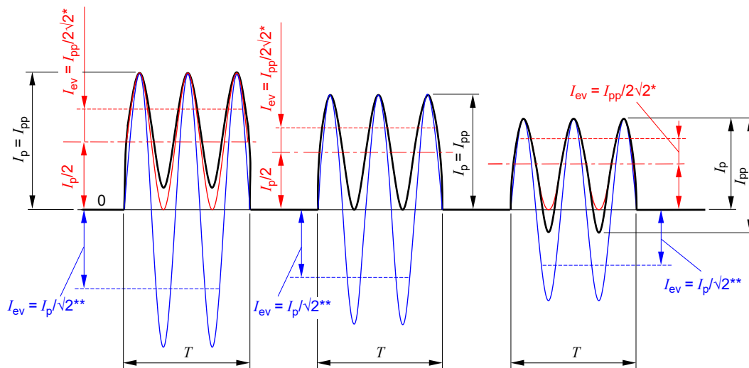
a) Combined waveforms of various ratios AC to DC together with rectangle pulse for shock duration >1,5 and <0,75 of the cardiac cycle
