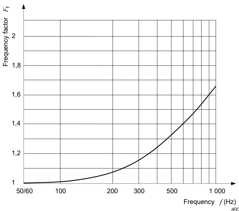
Figure 2 – Variation of the threshold of let-go within the frequency range 50/60 Hz to 1 kHz
