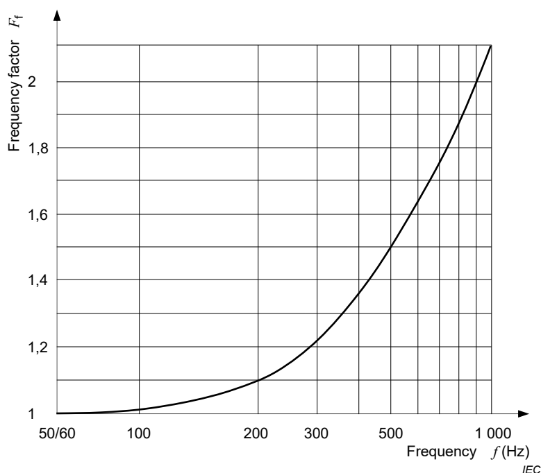
Figure 1 – Variation of the threshold of startle reaction within the frequency range 50/60 Hz to 1 kHz
