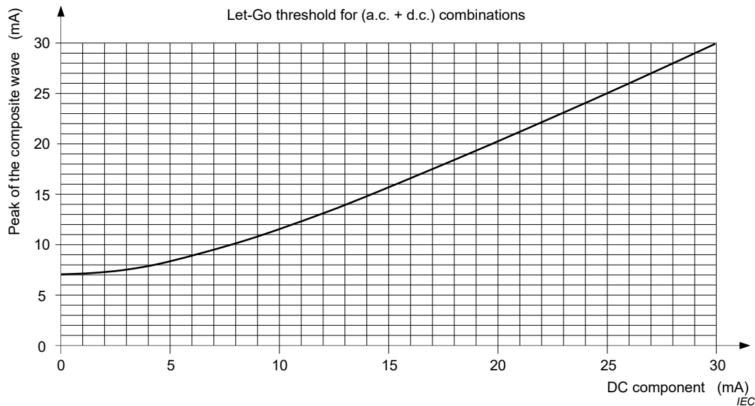
597 Figure 9 – 99,5 percentile let-go threshold for combinations 598 of 50/60 Hz sinusoidal alternating current and direct current
