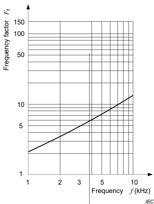
474 Figure 4 – Variation of the threshold of startle reaction 475 within the frequency range 1 kHz to 10 kHz
