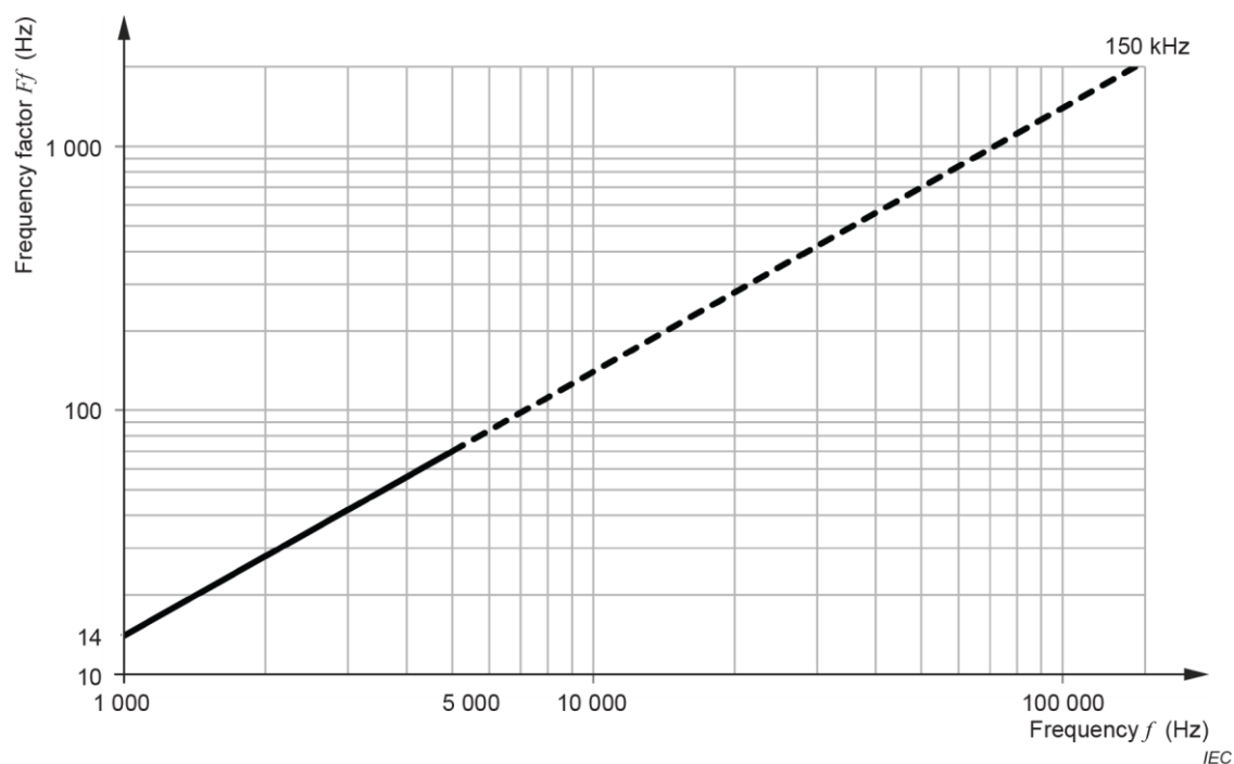
Figure 6 – Variation of the frequency factor of the threshold of ventricular fibrillation for continuous sinusoidal current for use from 1 kHz to a maximum of 150 kHz
