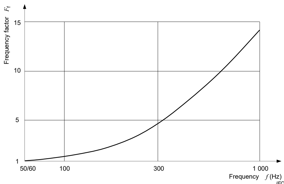
466 Figure 3 – Variation of the threshold of ventricular fibrillation within the frequency range 467 50/60 Hz to 1 kHz, shock durations longer than one heart period and longitudinal current paths 468 through the trunk of the body
