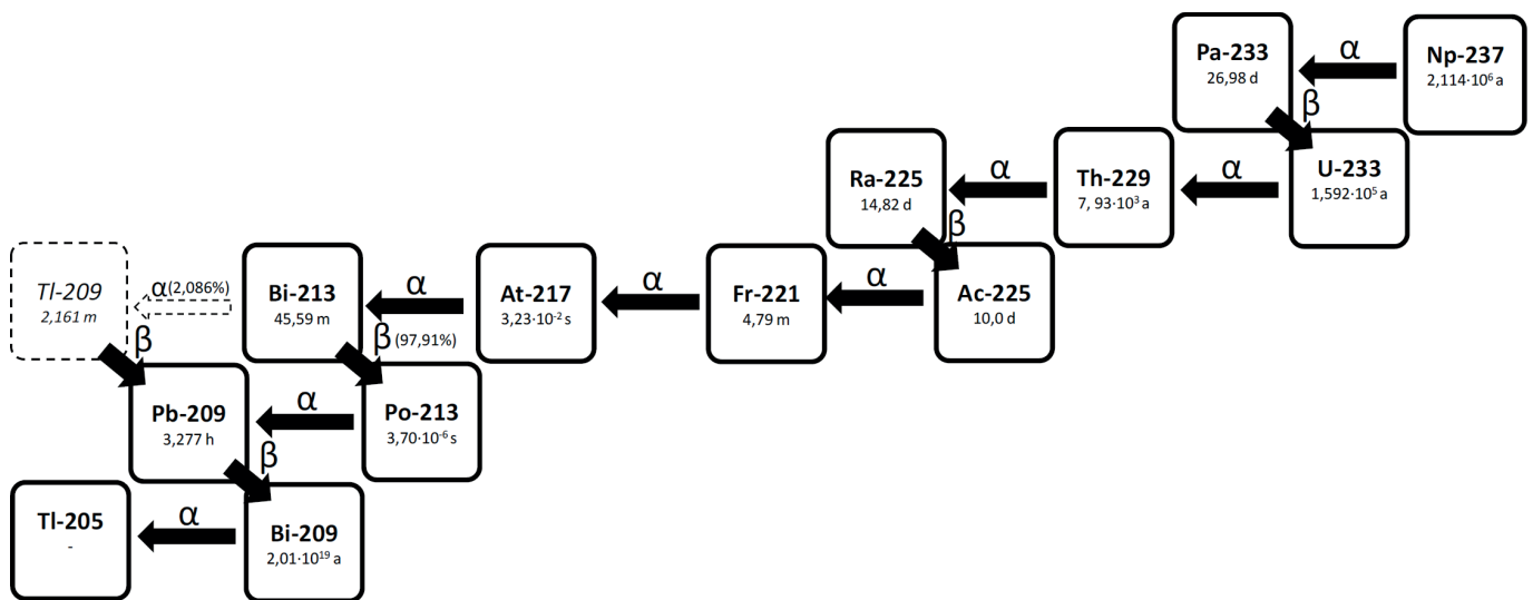
Figure 2 — ^{237}\text{Np} decay series
