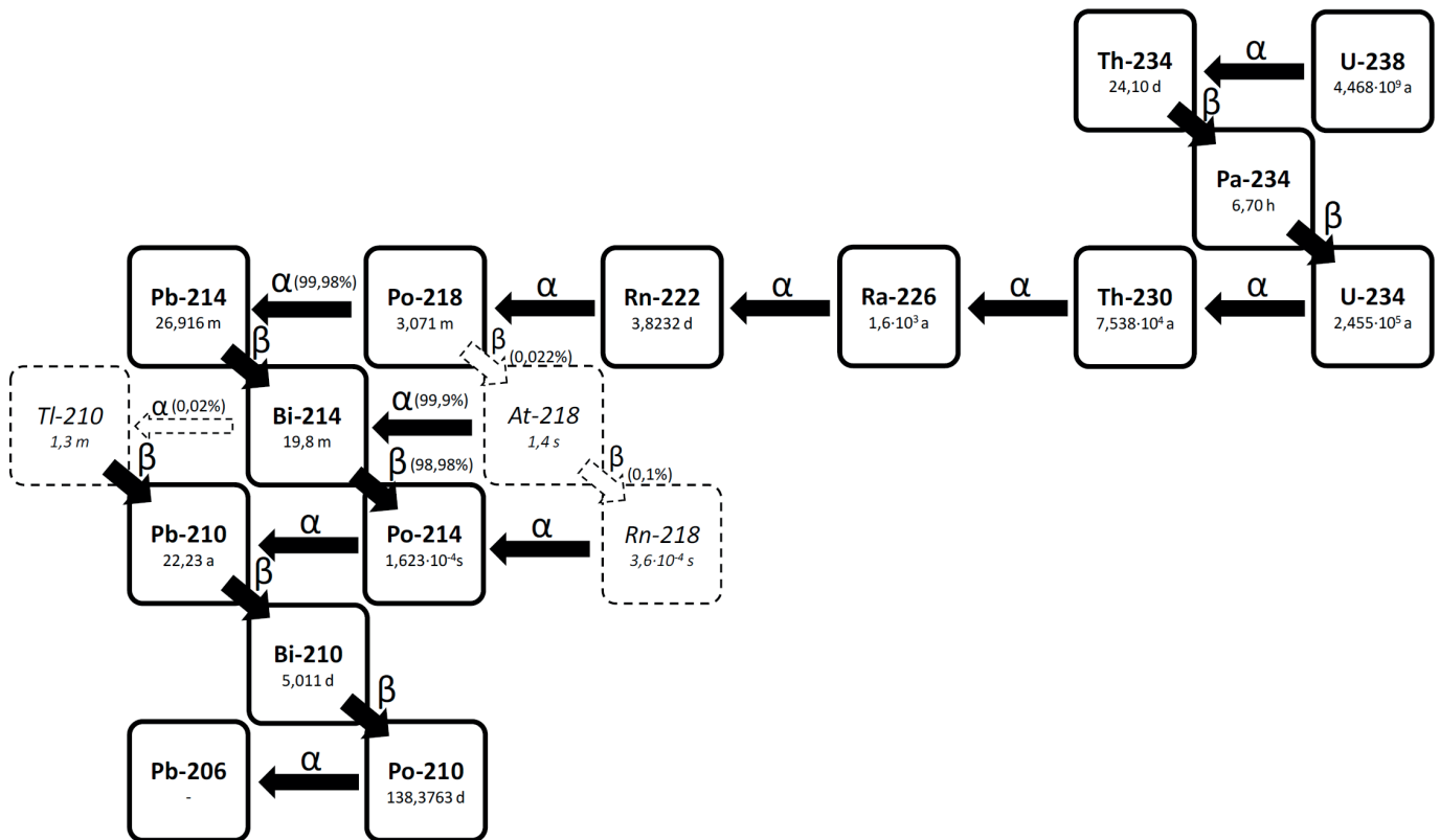
Figure 1 — ^{238}\text{U} decay series
