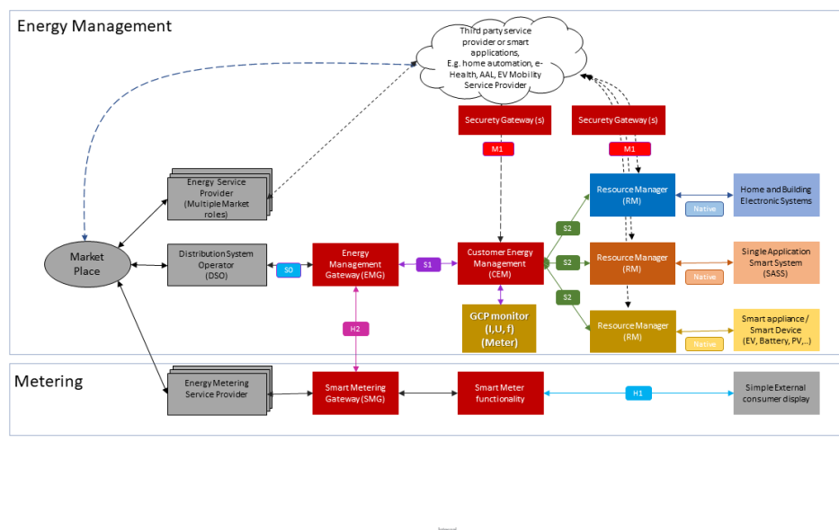
Figure 1 – Architectural overview of Premises smart grid system
