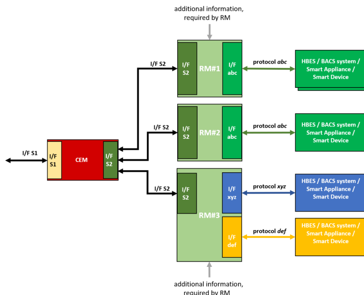
Figure 3 – Example Resource Manager and () / () /smart appliance/device combinations
