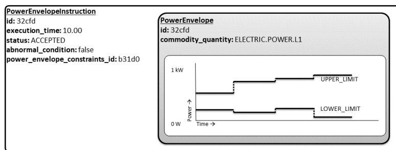
Figure 4 – Example of a PowerEnvelopeInstruction from the PowerEnvelope
