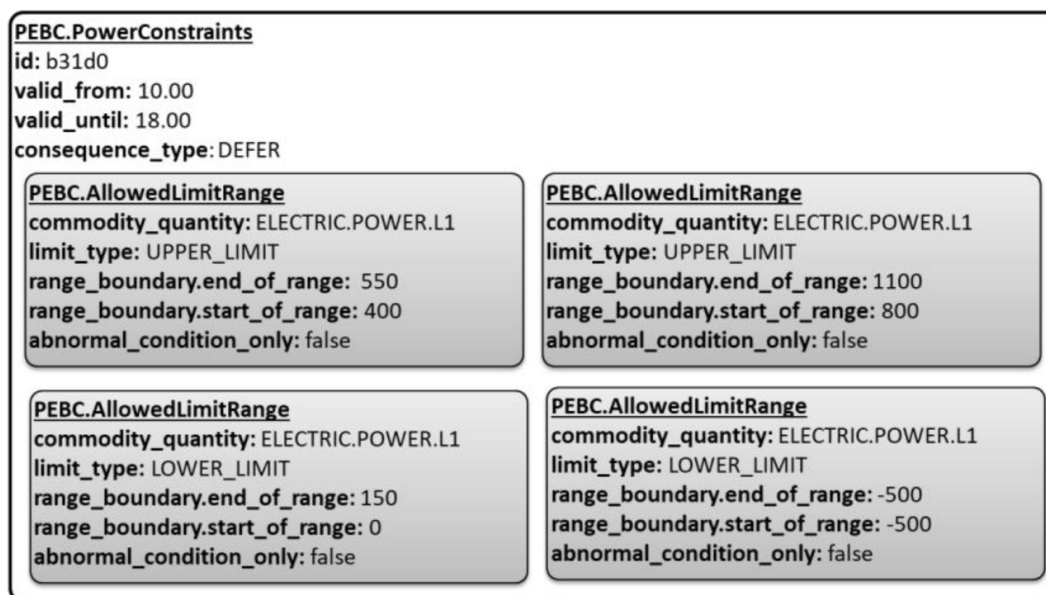
Figure 7 – Example of the PowerConstraints based on 6 b)
