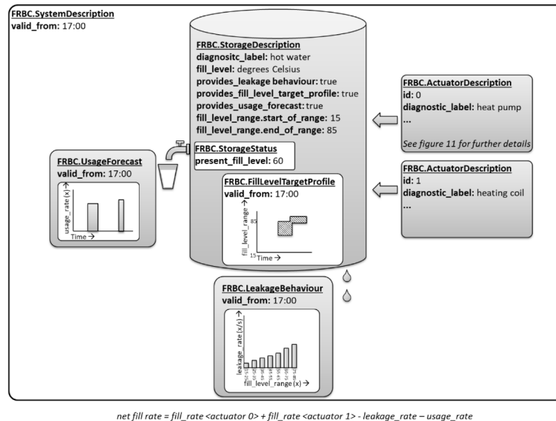
Figure 12 – Example for Fill Rate Based Control
