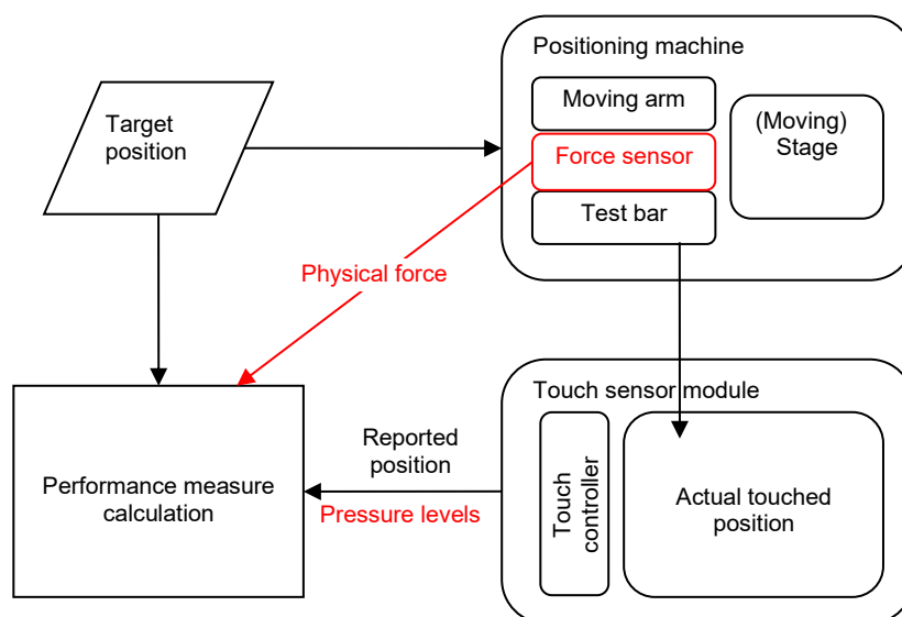
Figure 6 – Block diagram showing function and data added to Figure 2 in red for pressure characteristics measurement
