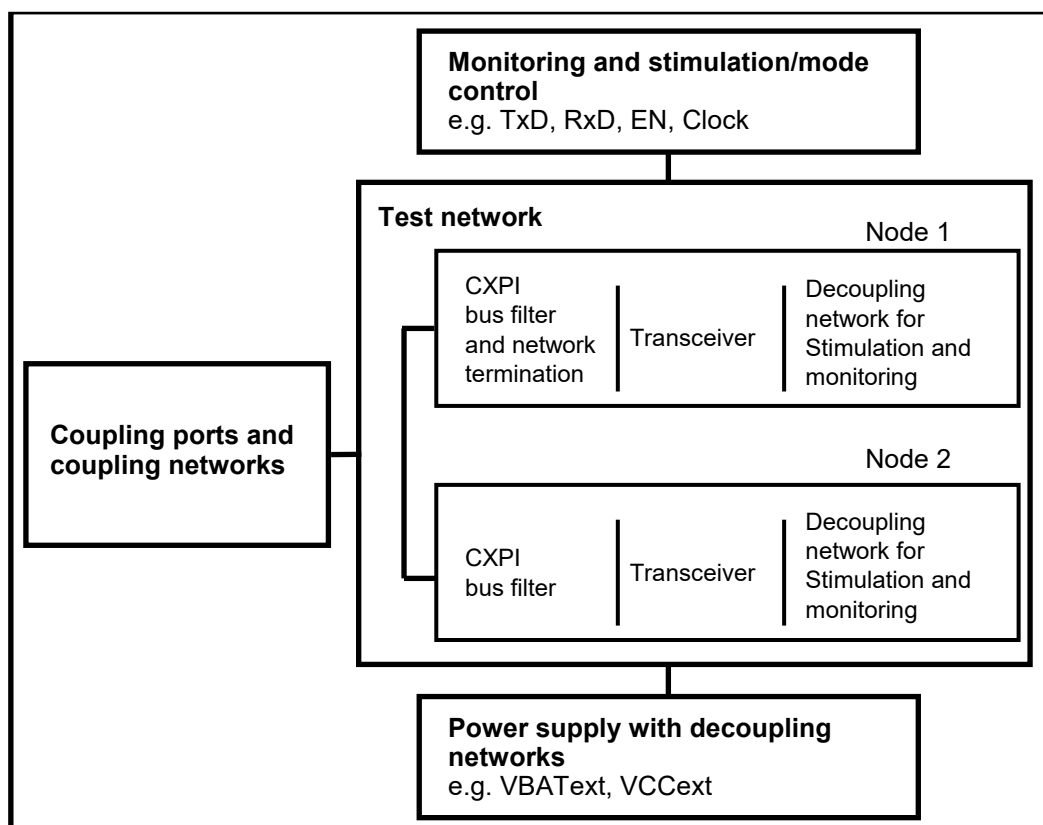
Figure 2 – General test configuration for tests in functional operation modes
