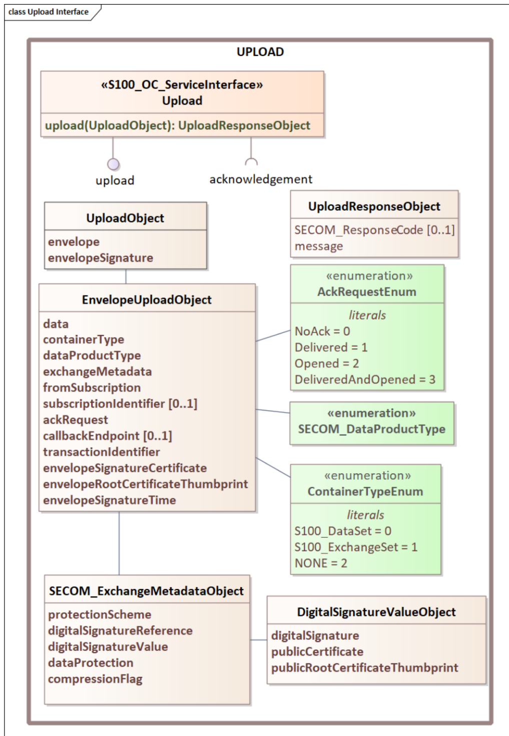
Figure 11 – Upload interface UML diagram
