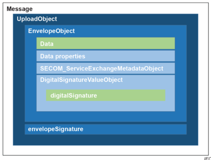
Figure 3 – Illustration of what parts of the message are protected by the two signatures
