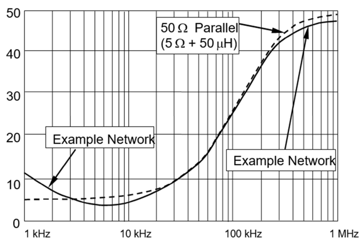
Figure 4 — Example of artificial network covering the frequency ranges 9 kHz to 95 kHz and 95 kHz to 526,5 kHz
