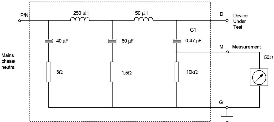
Figure 2 — Artificial mains network 3 kHz to 9 kHz
