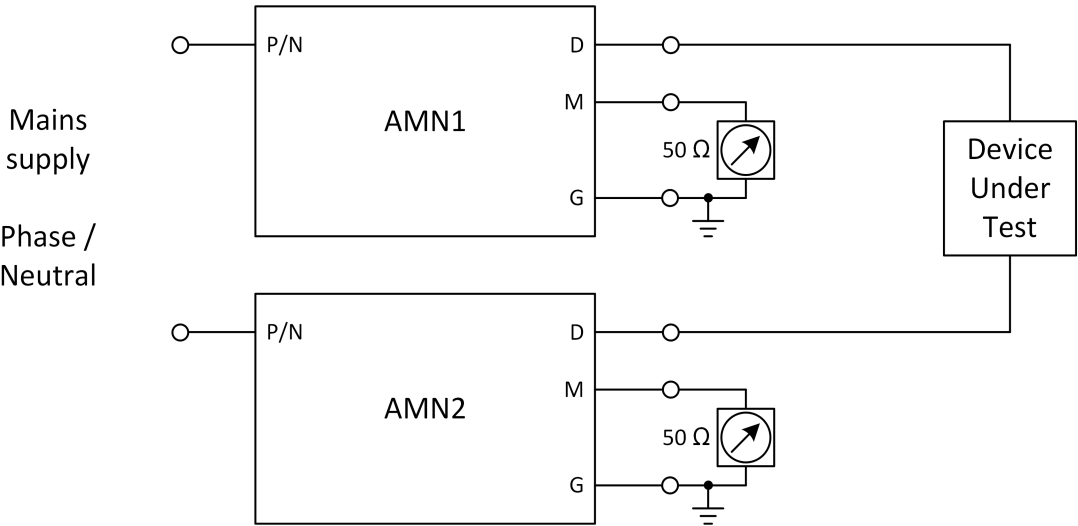
Figure 3 — Measurement of output signal voltage level (single phase)
