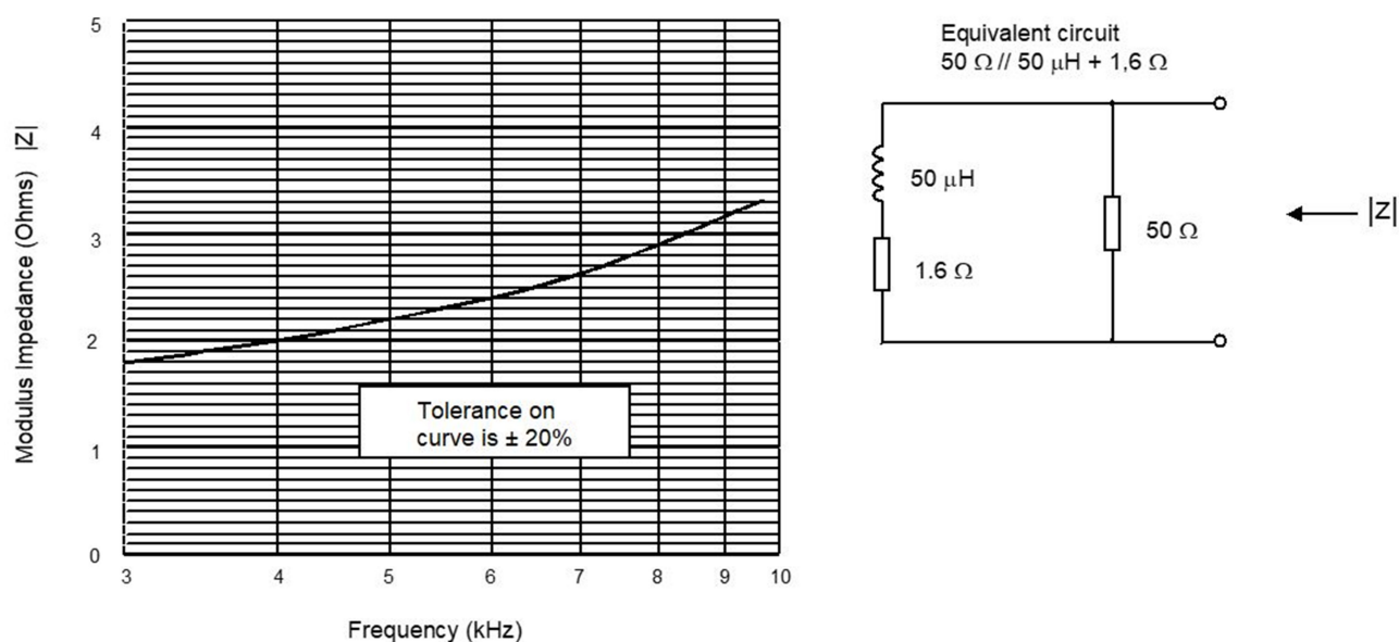
Figure 1 — Idealised equivalent circuit model – DUT port impedance
