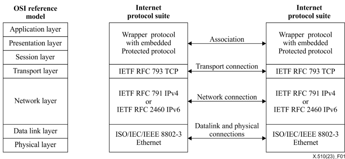
Figure 1 – Communication model
