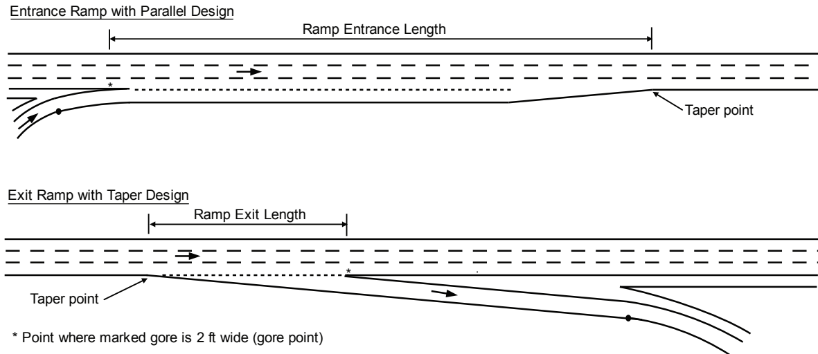
Figure 18-3. Freeway Speed-Change Lane Length
