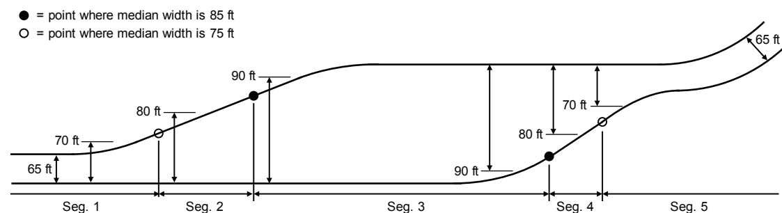
Figure 18-11. Segmentation for Varying Median Width
