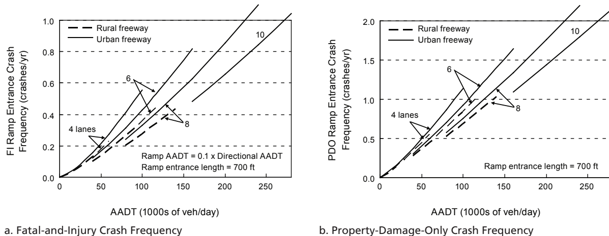
Figure 18-14. Graphical Form of the SPFs for Ramp Entrance Speed-Change Lanes
