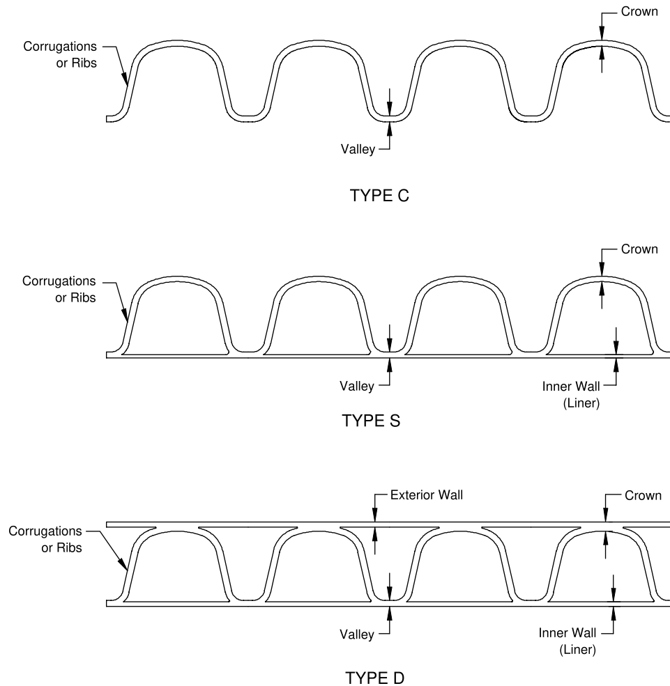
Figure 1 —Types of Corrugated Polypropylene Pipe
