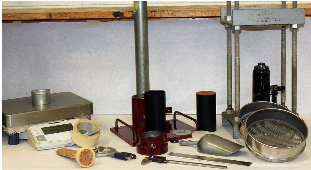
Figure 1 —Overview Photo of All PM Device Apparatus Items
