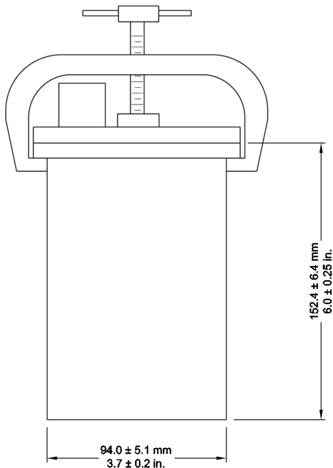
Figure 1 —Metal Still
