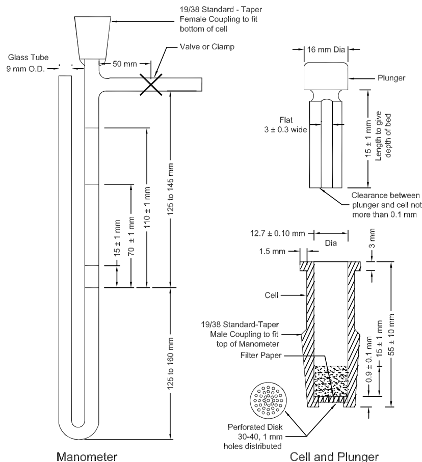
Figure 1 —Blaine Air Permeability Apparatus
