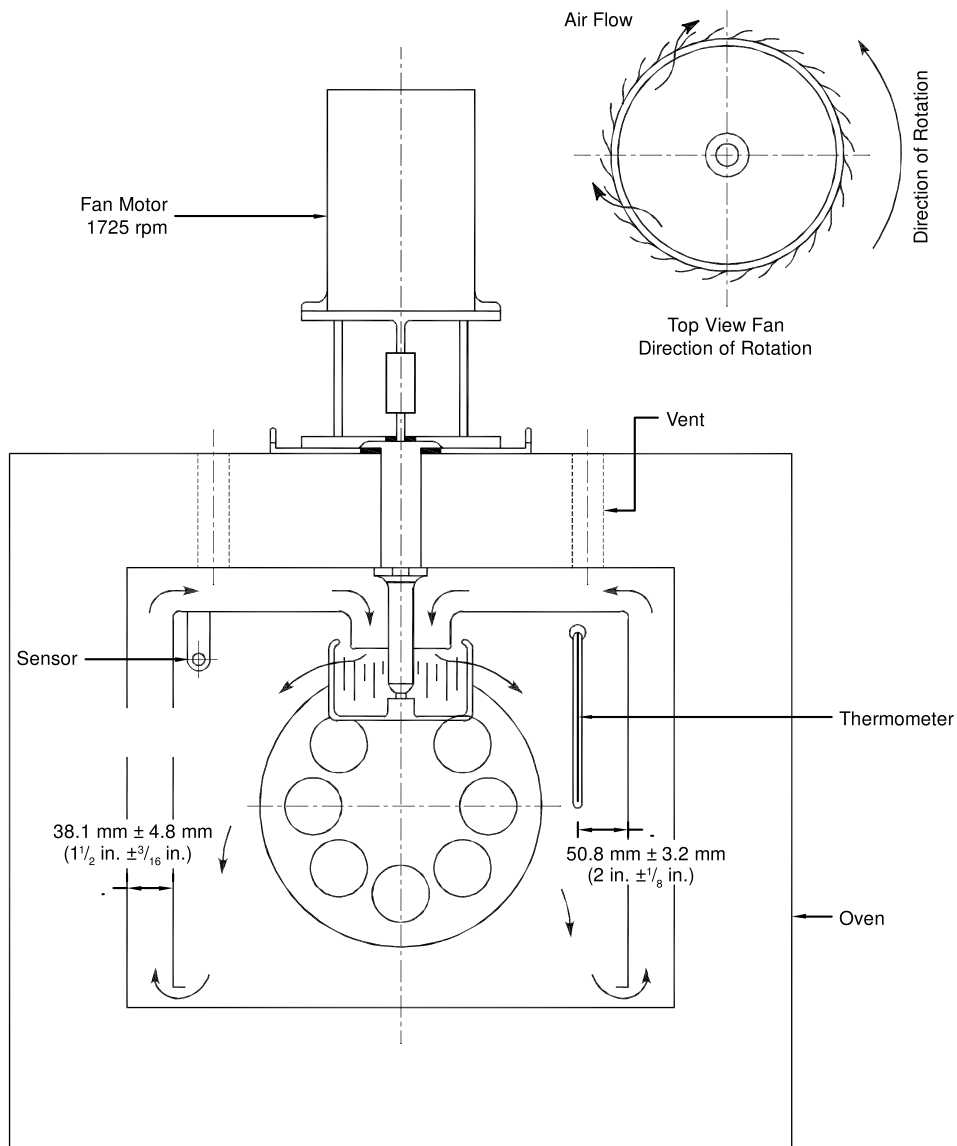
Figure 1 —Schematic of Air Flow Front View
