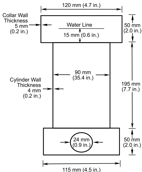
Figure 1 —Riser Cylinder
