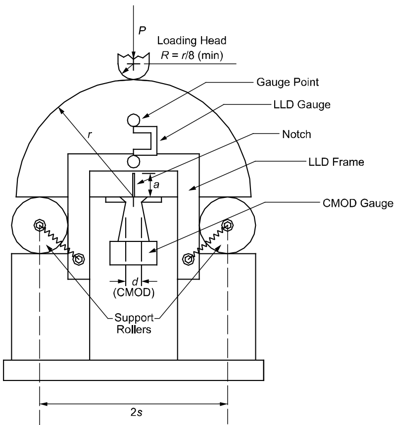
Figure 1 —SCB Loading Setup for Front and Back Sides of Test Specimen
