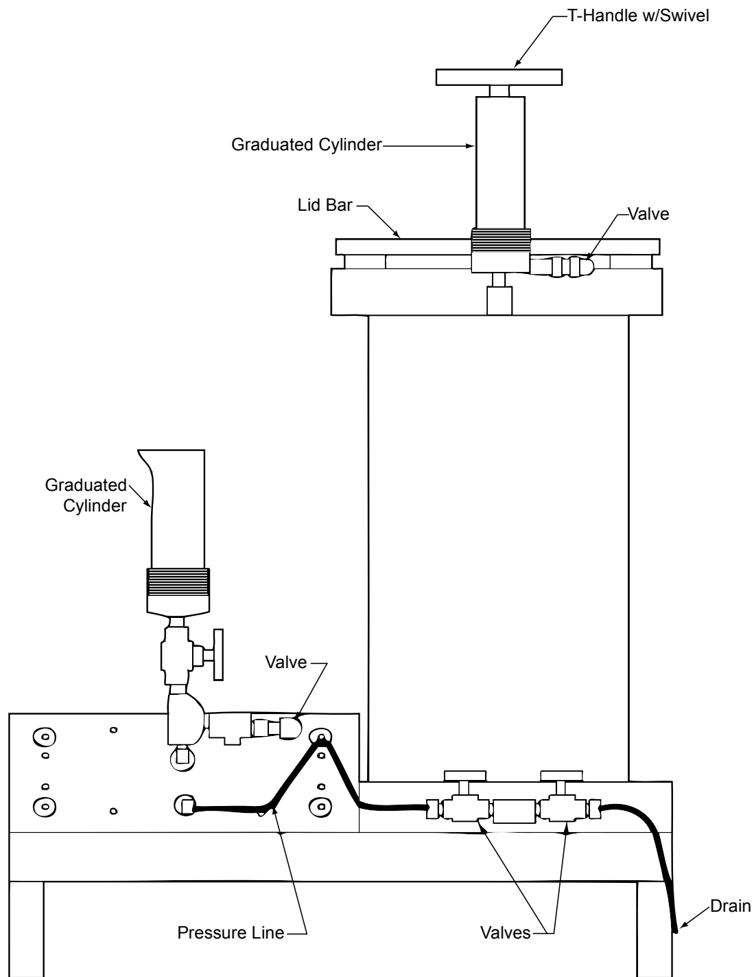
Front View of Test Chamber
