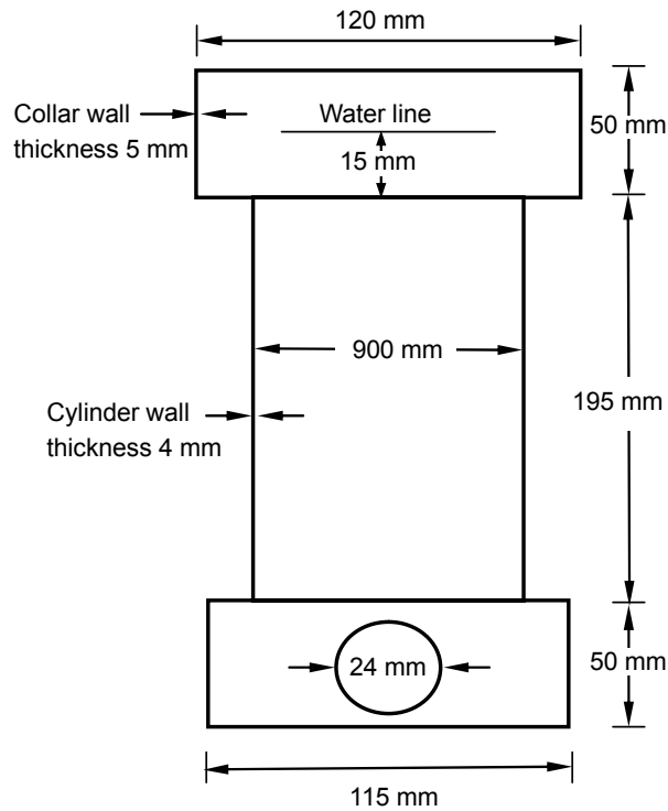
Figure 1 —Riser Cylinder
