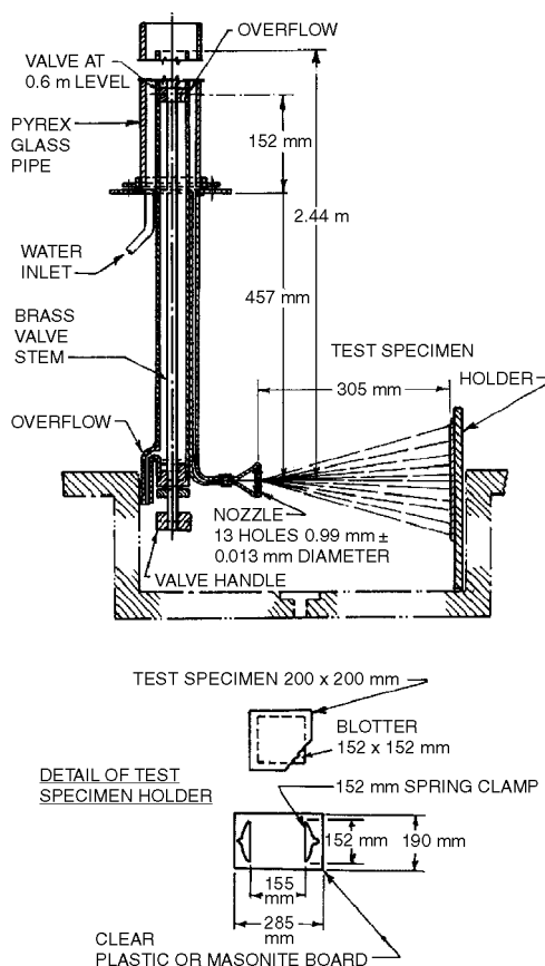
Fig. 2—Rain tester, structural details.
