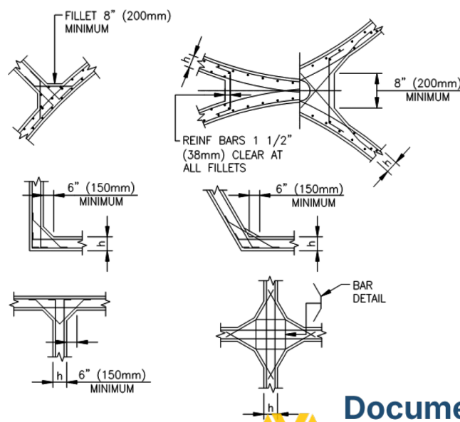
Fig. R6.2.1a—Reinforcement pattern at intersections
