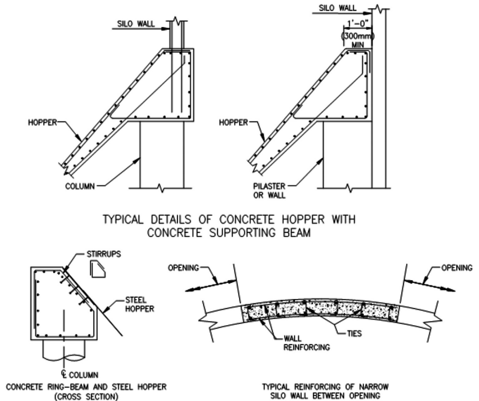
Fig. R6.2.1b—Miscellaneous details.
