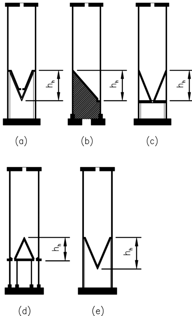
Fig. 6.1.1—Examples of vertical cross sections of silos used to determine the height of the hopper. Other configurations are possible.
