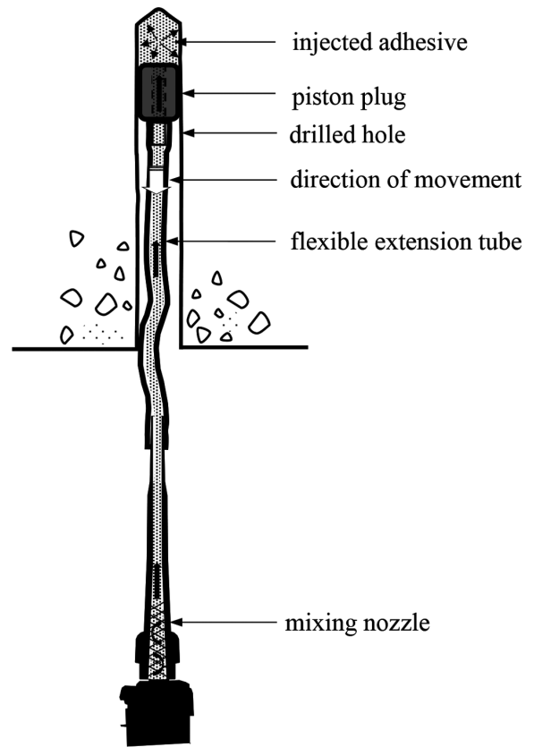
Fig. 2.2—Use of piston plug for adhesive injection.
