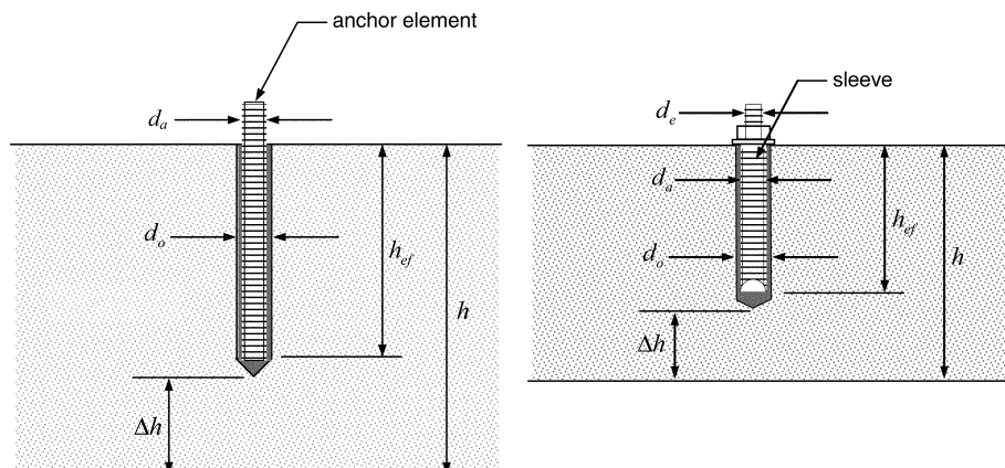
Fig. 2.1—Adhesive anchor dimensional parameters.
