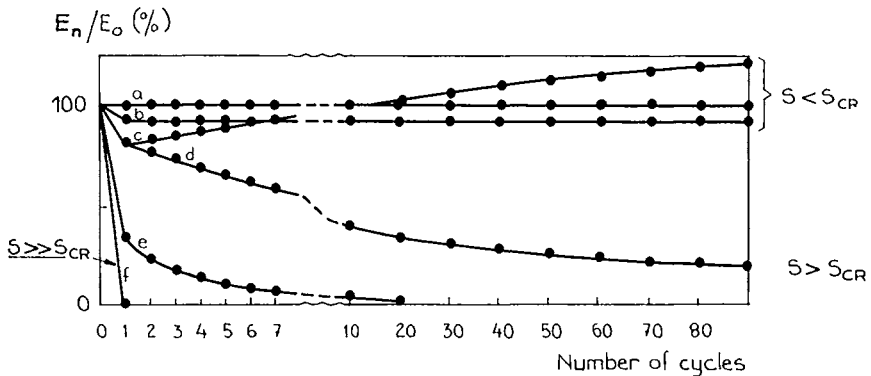
Fig. 2--Principles for variation of dynamic Young's modulus with number of cycles when the degree of saturation is constant
