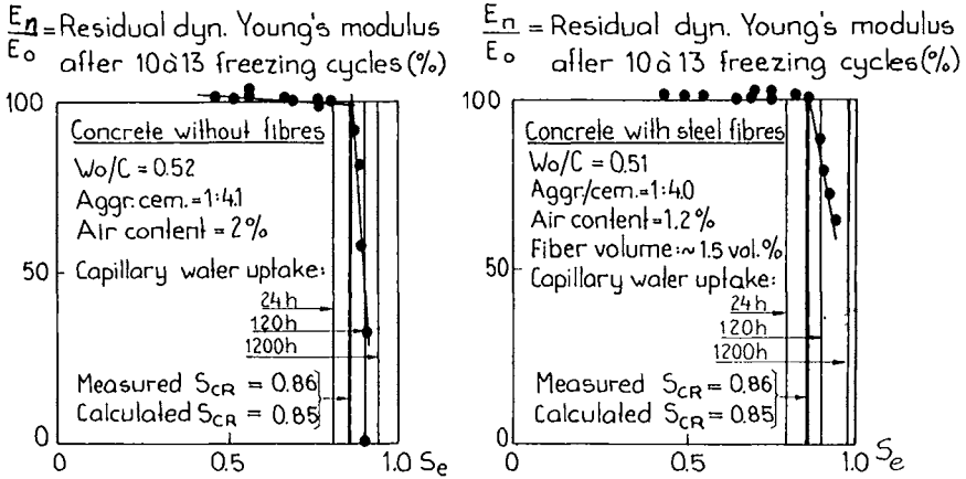
Fig. 1--Experimental and theoretical critical degrees of saturation of a concrete with and without steel fibers. Capillary water uptake indicated in the figure
