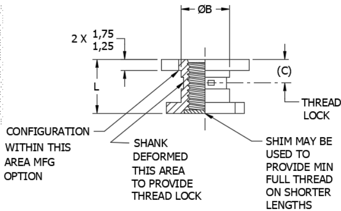
SHIMMED STYLE FOR SHORTER LENGTHS
