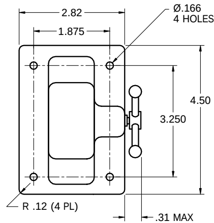
-2 PUSH SWITCH COVER
