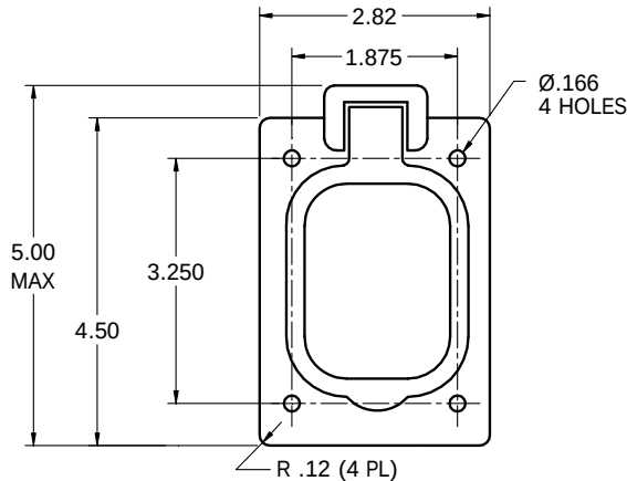
-3 DUPLEX RECEPTACLE COVER
