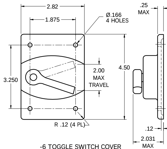
-6 TOGGLE SWITCH COVER
