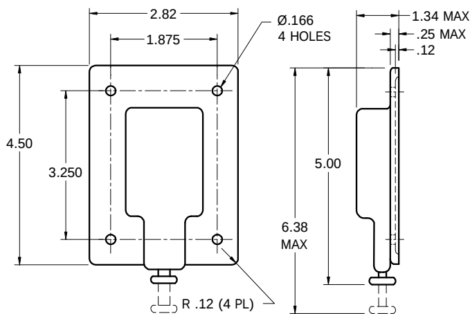
-7 ROD OPERATED TOGGLE SWITCH COVER
