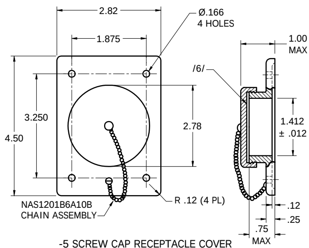
-5 SCREW CAP RECEPTACLE COVER
