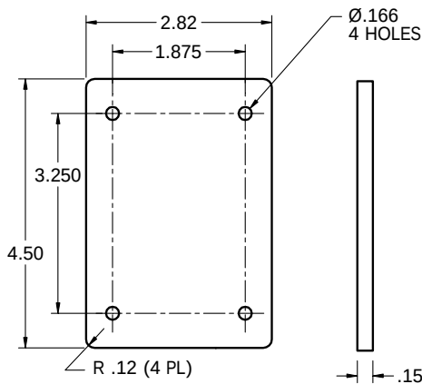
-11 BLANK COVER
