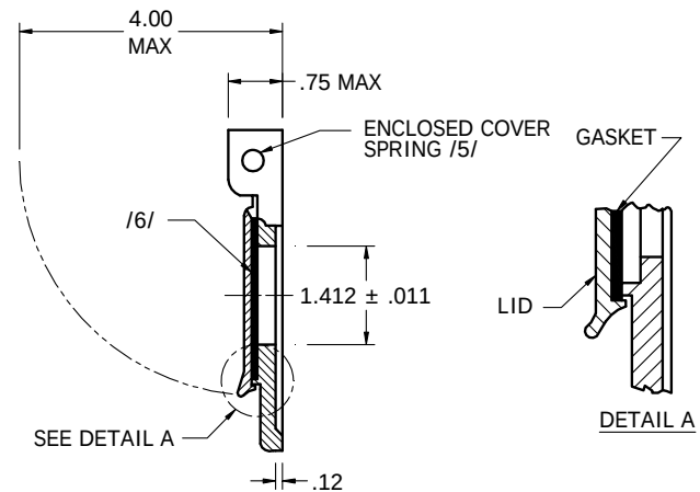
-4 SINGLE RECEPTACLE COVER
