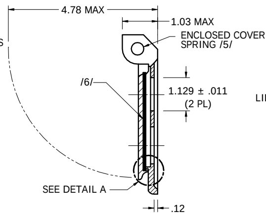
-3 DUPLEX RECEPTACLE COVER
