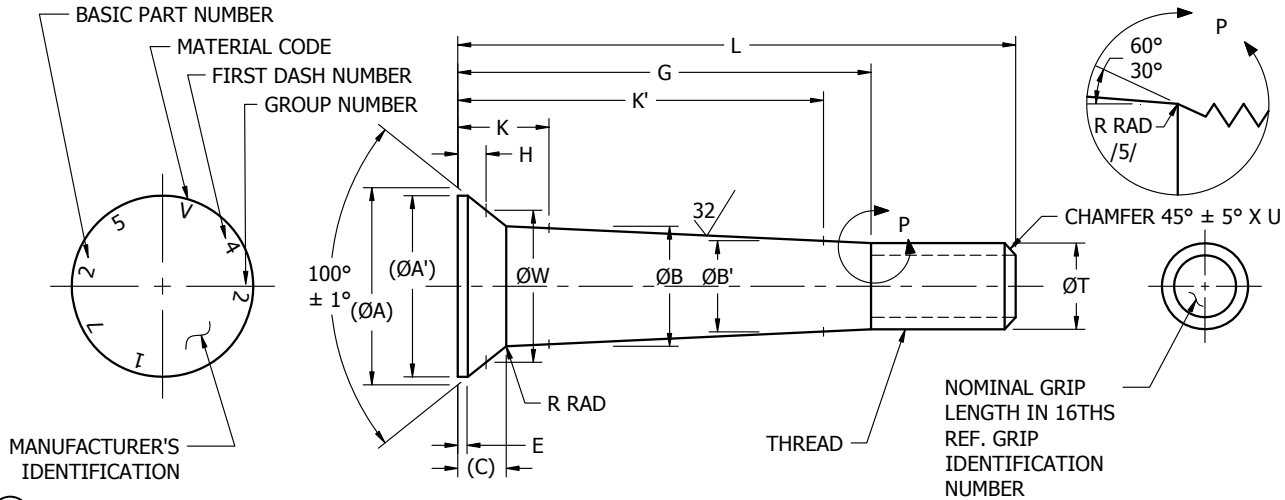
FIGURE 1 - FASTENER TABLE I - DIMENSIONS
