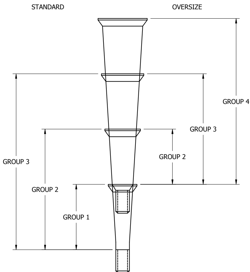
FIGURE 2 – GROUP ARRANGEMENT
