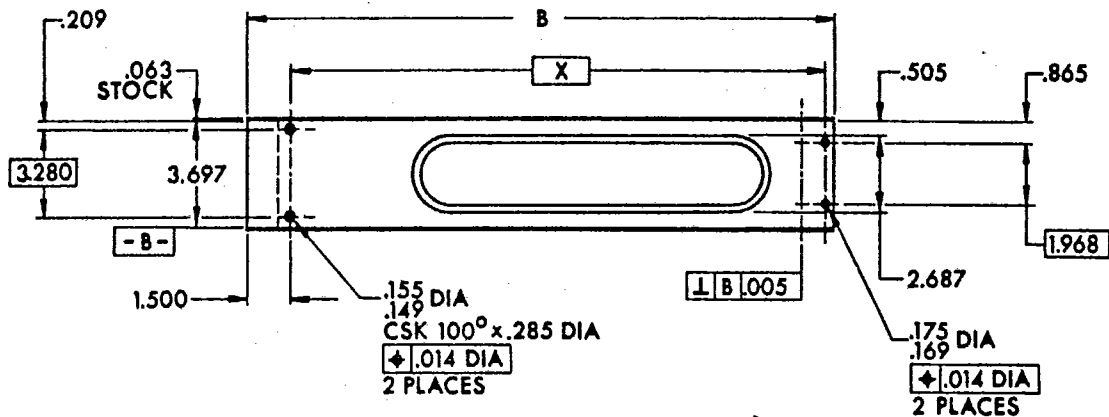
MOUNT HOLE OPTION "X"
