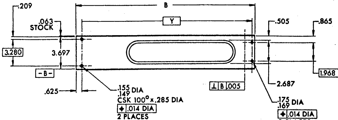
MOUNT HOLE OPTION "Y"
