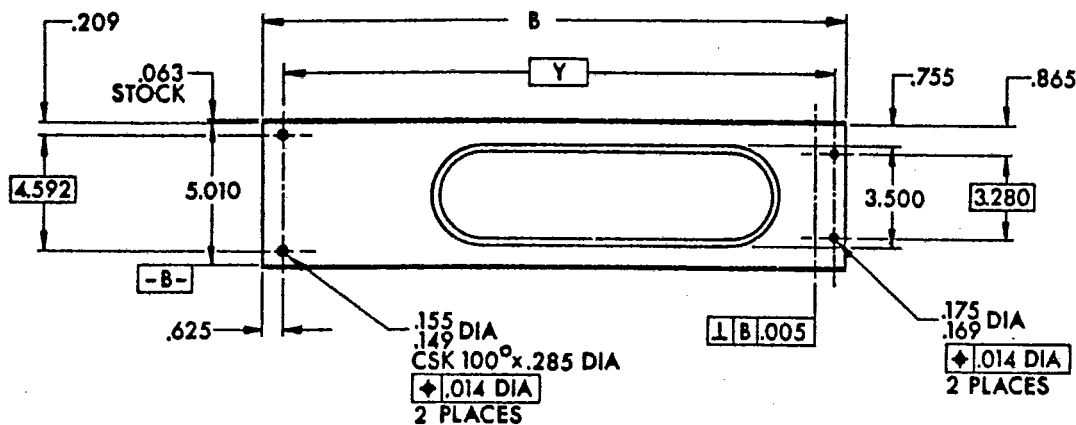
MOUNT HOLE OPTION "Y" \Delta 7
