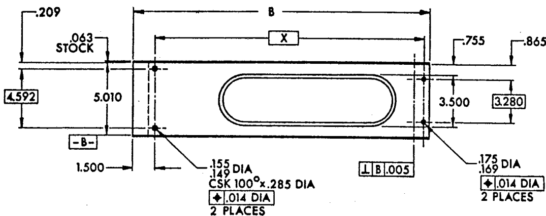
MOUNT HOLE OPTION "X" \Delta 7
