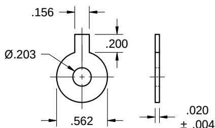
CONFIGURATION F DASH NUMBER "13"
