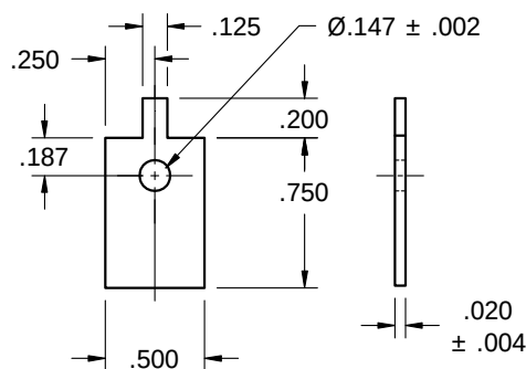
CONFIGURATION E DASH NUMBER "12"
