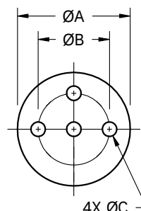
CONFIGURATION K DASH NUMBER "19" AND "39"
