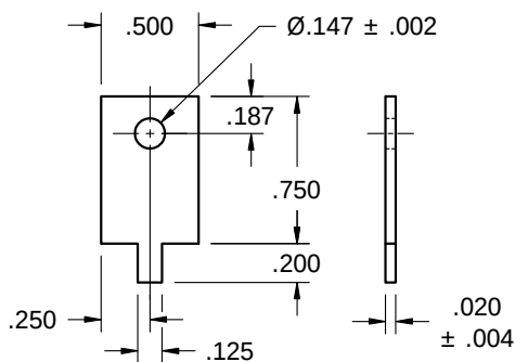
CONFIGURATION D DASH NUMBER "11"
