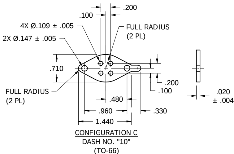
FIGURE 2 – CONFIGURATIONS B AND C
