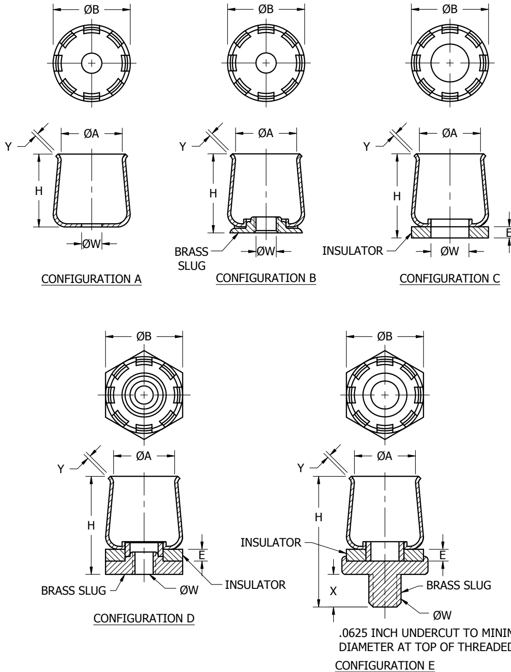
FIGURE 1 – CONFIGURATIONS AND DIMENSIONS
