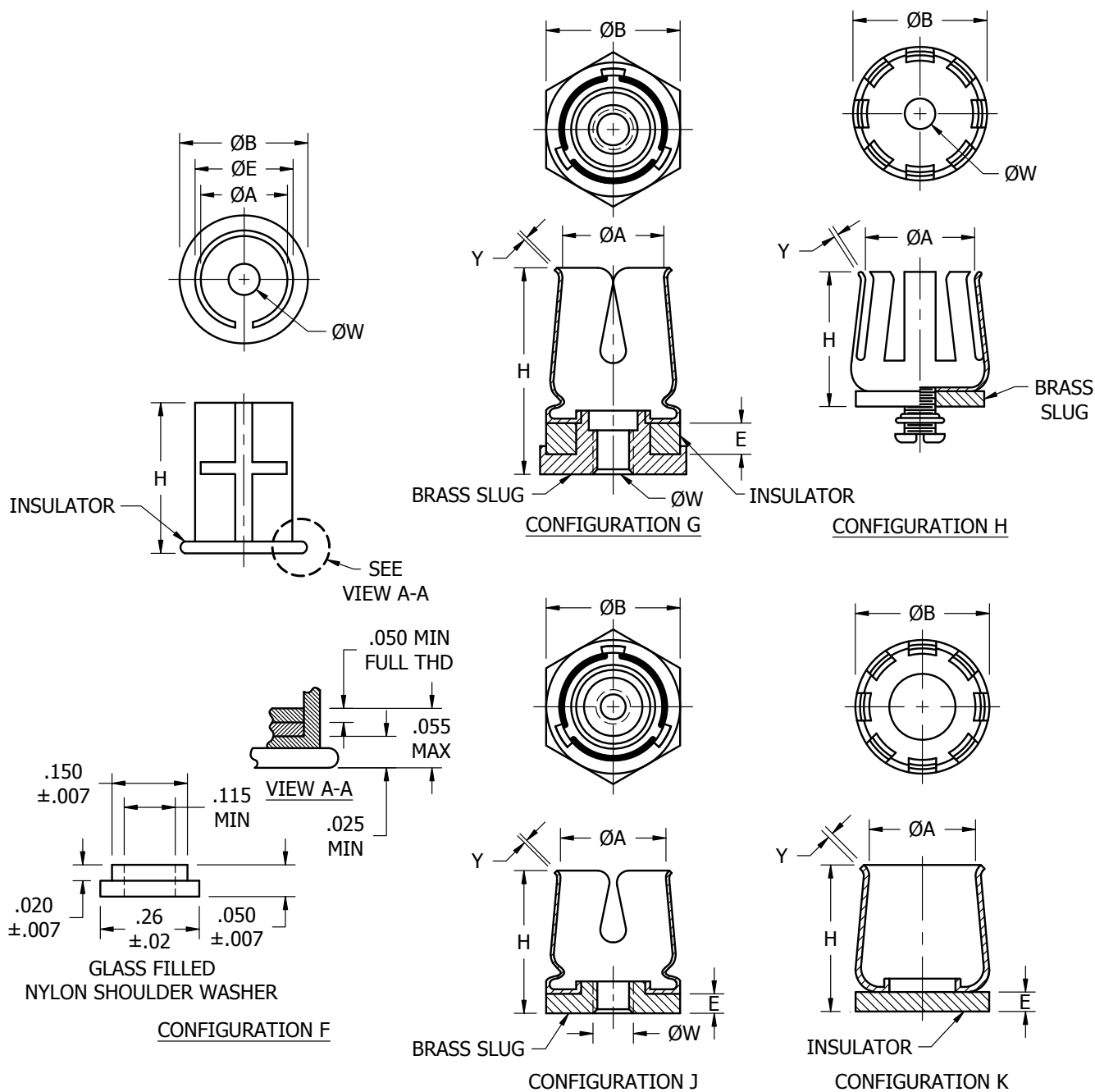
FIGURE 1 – CONFIGURATIONS AND DIMENSIONS (CONT)
