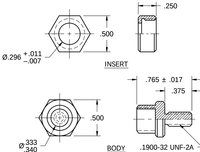
CONFIGURATION D DASH NUMBER "04"
