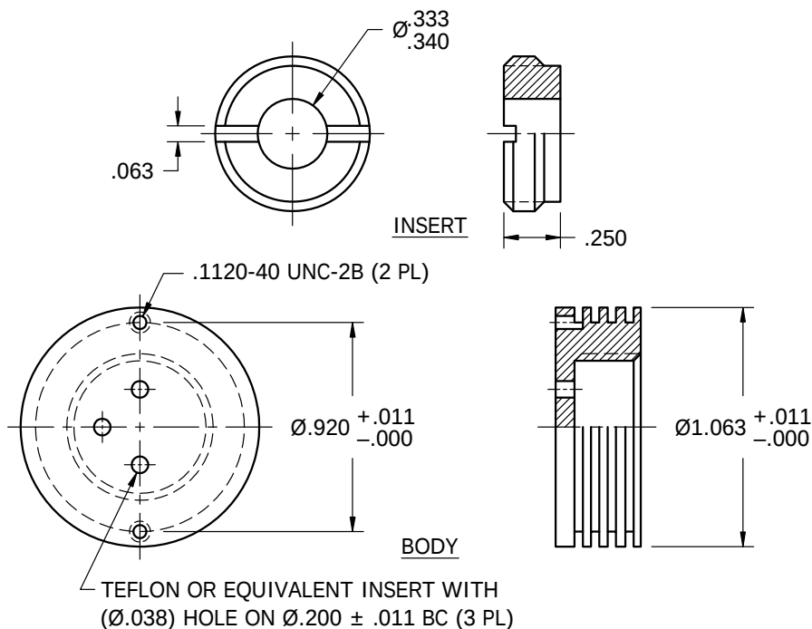
CONFIGURATION C DASH NUMBER "03"
