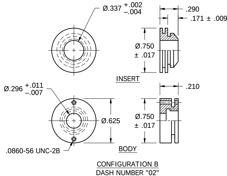
FIGURE 1 – CONFIGURATIONS AND DIMENSIONS
