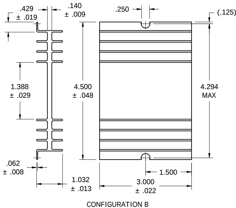
FIGURE 1 – CONFIGURATIONS AND DIMENSIONS
