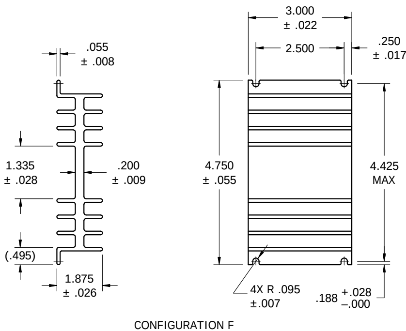
FIGURE 1 – CONFIGURATIONS AND DIMENSIONS (CONTINUED)
