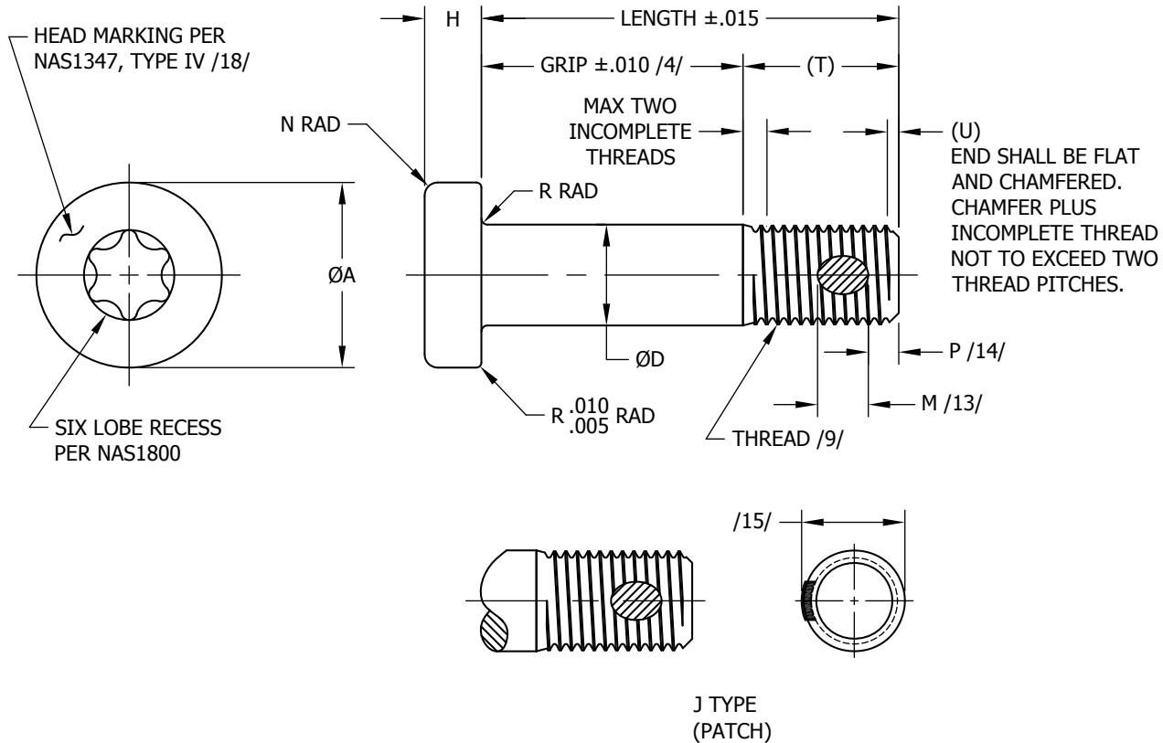
FIGURE 1 – BOLT CONFIGURATION
