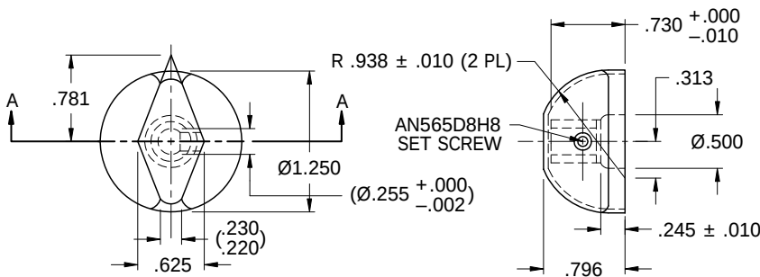
-1A KNOB ASSEMBLY, FUEL FLOW, FLATTED SHAFT
