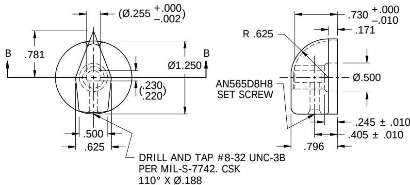
-1B KNOB ASSEMBLY, POINTER, FLATTED SHAFT
