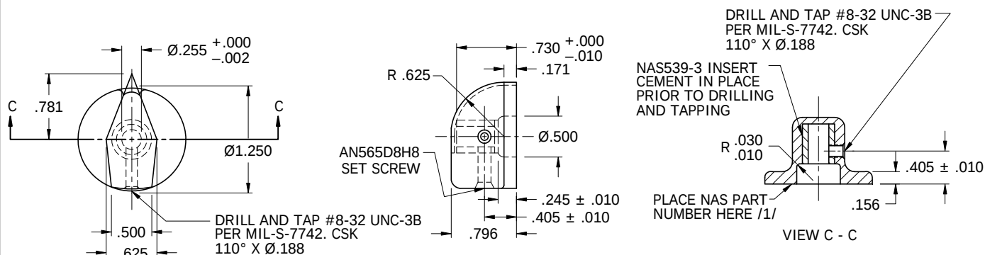
-1C KNOB ASSEMBLY, POINTER, ROUND SHAFT
