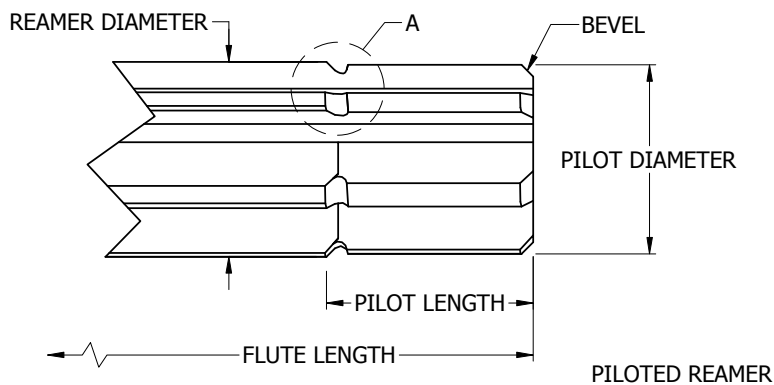
PILOTED REAMER
