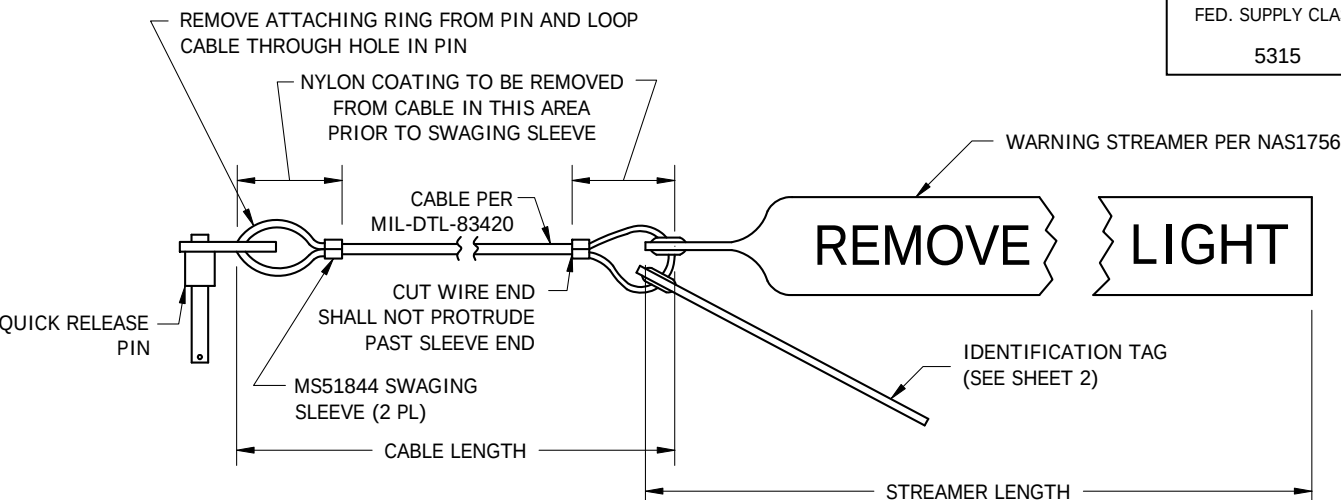
FIGURE 1 – PIN, QUICK RELEASE WITH WARNING STREAMER ASSEMBLY
