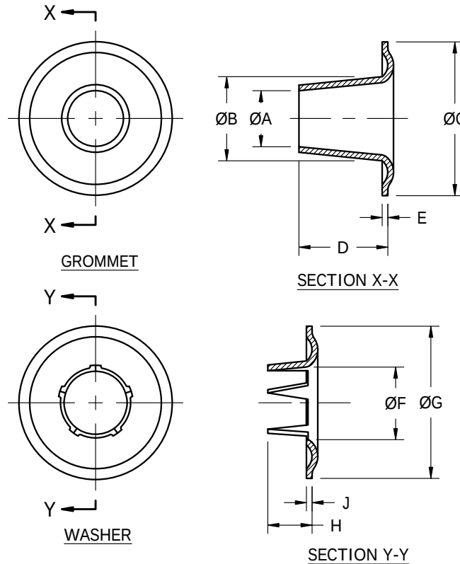
FIGURE 1 – GROMMET, METALLIC, PLAIN, WITH TOOTHED WASHER (TYPE II)
