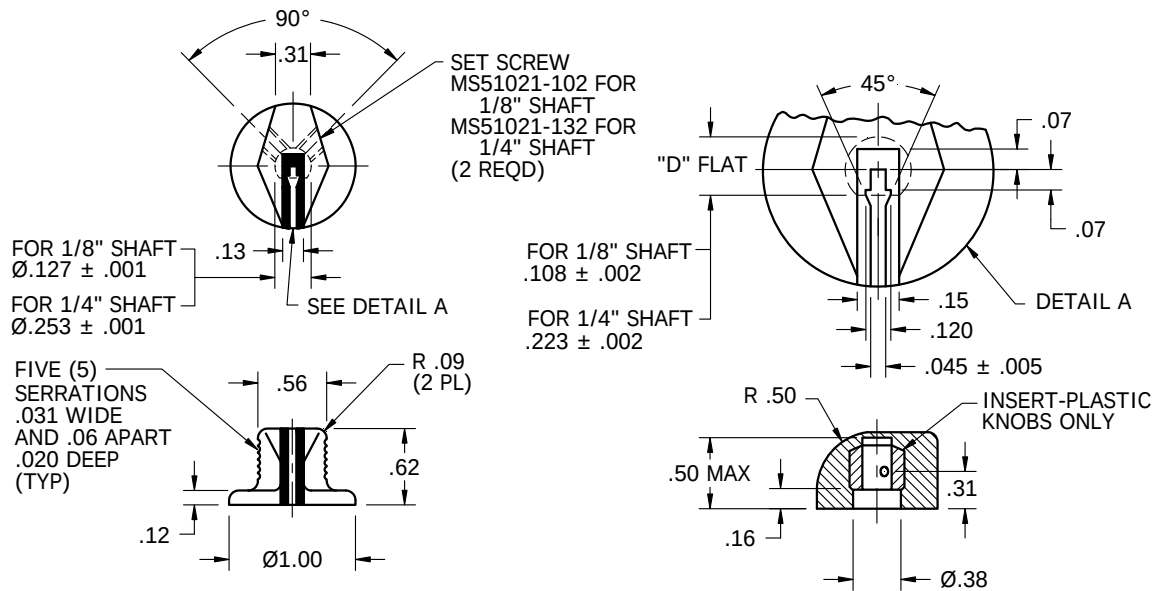
FIGURE 2 – KNOB, STYLE B & F
