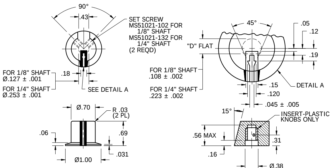
FIGURE 3 – KNOB, STYLE C & G
