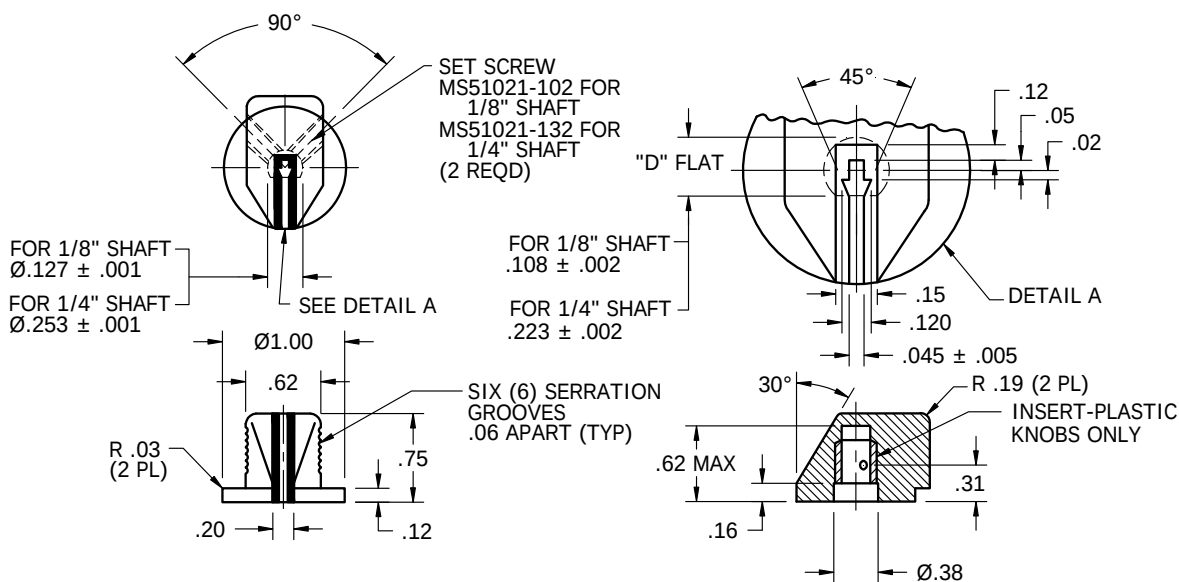
FIGURE 4 – KNOB, STYLE D & H
