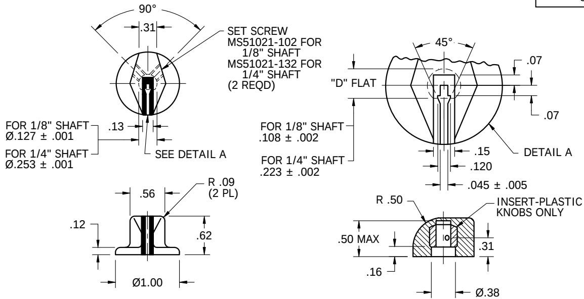
FIGURE 1 – KNOB, STYLE A & E
