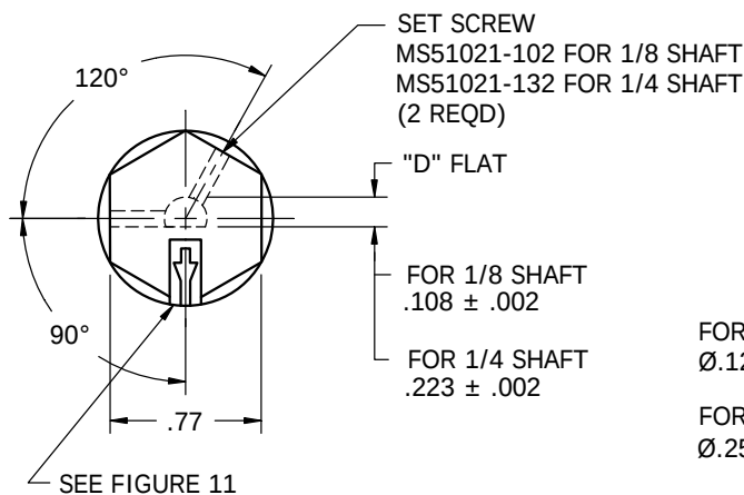
FIGURE 5 – KNOB, STYLE E OR Q
