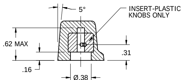
FIGURE 4 – KNOB, STYLE D OR P
