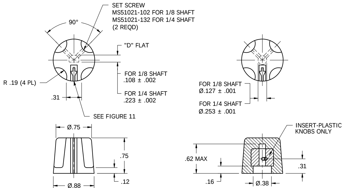
FIGURE 2 - KNOB, STYLE B OR M
