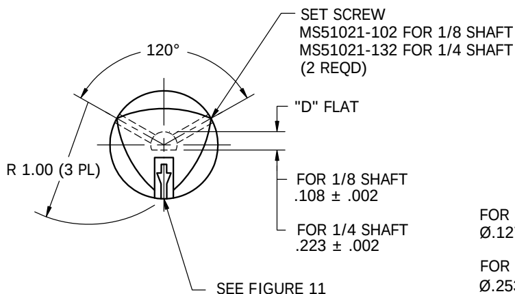
FIGURE 3 – KNOB, STYLE C OR N
