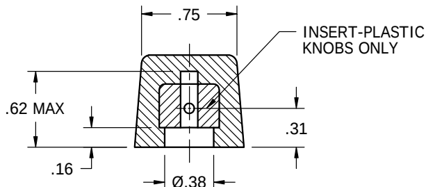
FIGURE 6 – KNOB, STYLE F OR R
