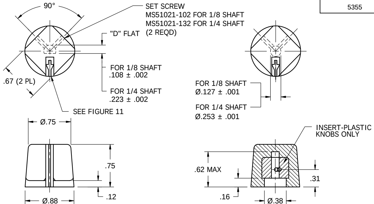
FIGURE 1 - KNOB, STYLE A OR L
