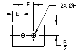
FIGURE 2 - TWO MOUNTING HOLES
