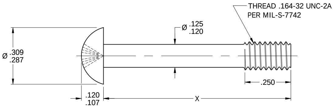
FIG 2. CROSS-RECESSED HEAD
