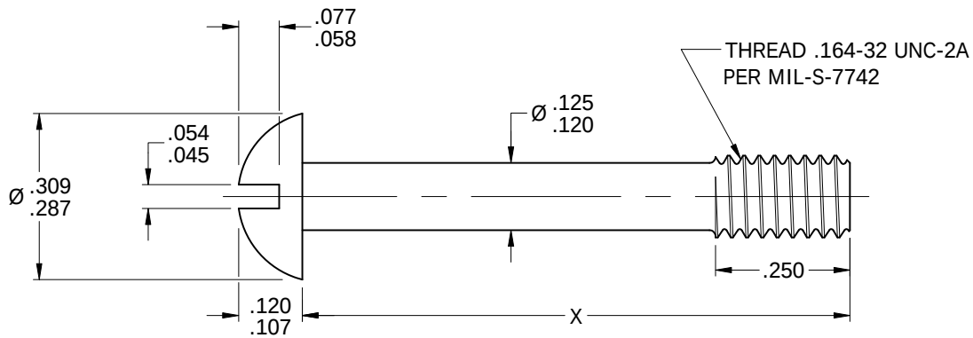
FIG 1. SLOTTED HEAD /6/
