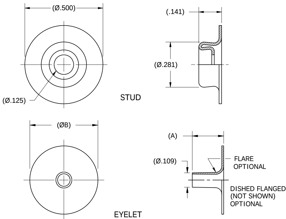
FIGURE 2 – STUD AND EYELET
