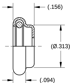
FIGURE 1 – BUTTON AND SOCKET
