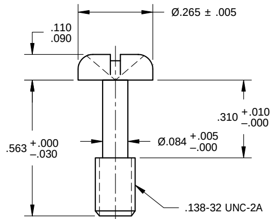
"-9", "-11" CAPTIVE SCREW, PAN HEAD, CRUCIFORM
