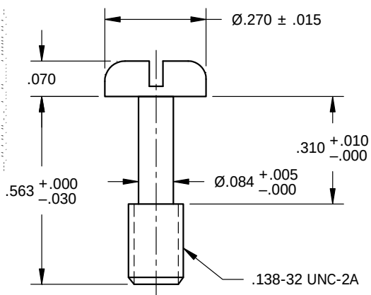
"-4", "-7" CAPTIVE SCREW, PAN HEAD, SLOTTED
