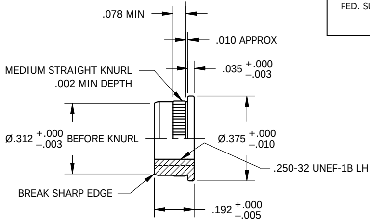
"-2" COLLAR
