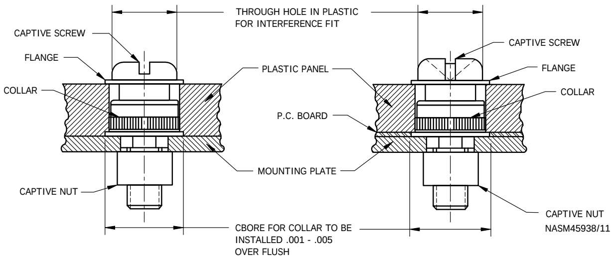
ASSEMBLY - TYPE IV & TYPE VI INSTALLATION
