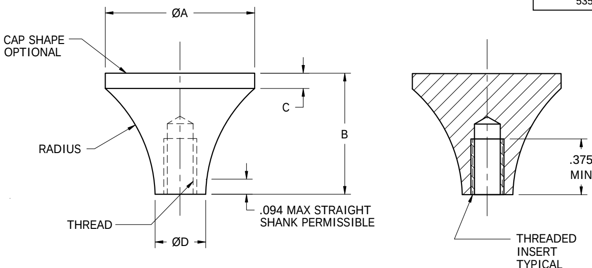
FIGURE 1 – KNOB, CONTROL, TAPERED
