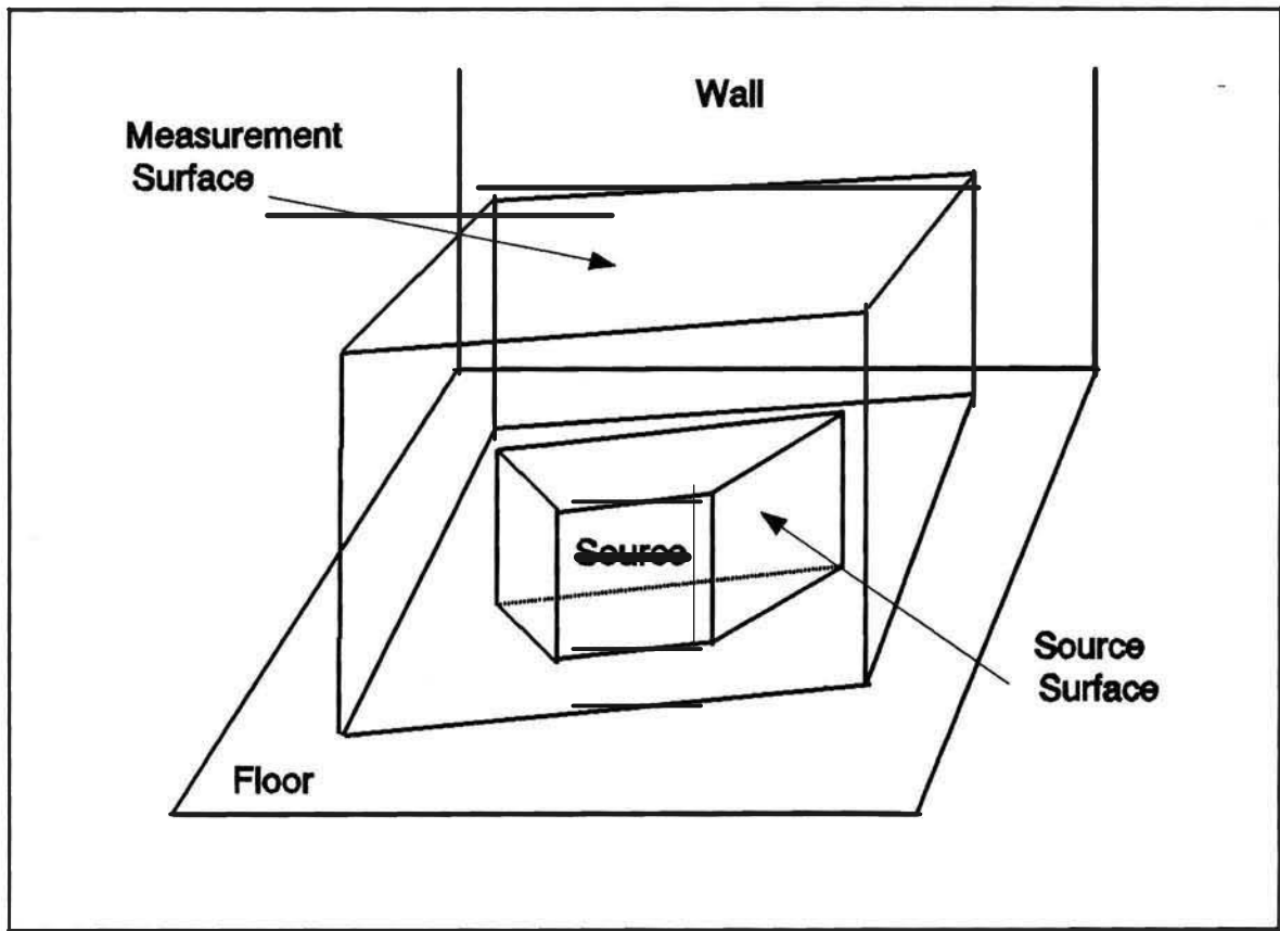
FIG. 1. Measurement surface. Plane surfaces are shown for illustration only. Regular, non-conformal measurement surface is shown.
